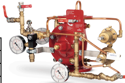
77DE-EL-PORV-PR-MR Manuel Reset
